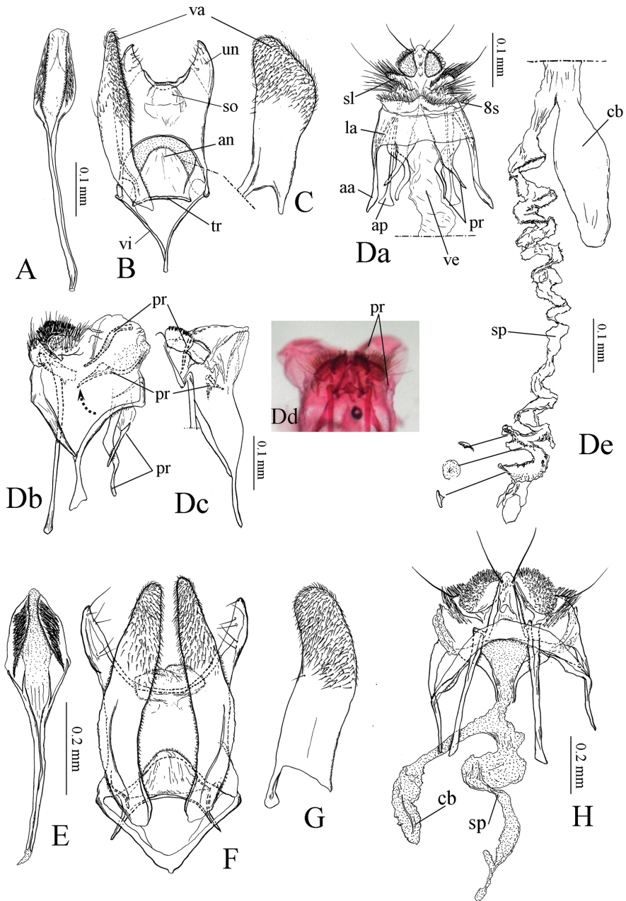
Figure 3. Genitalia of Coptotriche minuta and C. symlocosella . A–D: C. minuta . E–H: C. symlocosella . A, E Phallus, ventral view B, F Male genitalia, ventral view C, G Right valva, inner view D, H Female genitalia, ventral view Db, Dc, Dd Same, separated two pairs of prela towards posterior part Db Lateral view Dcd ventral view De Corpus bursae and ductus spermatheca. Abbreviations: aa: apophysis anterioris; an: anellus; ap: apophysis posterioris; cb: corpus bursae; la: lateral arm of 8th tergite; pr: prela; sl: setose lobe on 9th tergite; so: socius; sp: spermatheca; tr: transtilla; un: uncus; va: valva; vi: vinculum; ve: vestibulum; 8s: 8th sternite.
