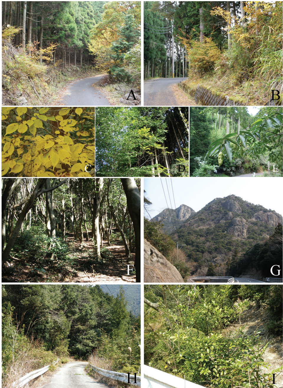
Figure 1. Habitats and hostplants of Coptotriche species. A–E C. minuta Diškus & Stonis, 2014, Soni, Nara Prefecture F–I C. symplacosella sp. n. A Habitat, Mitsuiyatani, Konagao, 710 m B Habitat, Nagano, 600 m C Leaves of Carpinus laxiflora at Nagano D Branches of C. japonica at Kumawata, Konagao E Leaves and fruits of C. japonica at Kumawata F Type locality, Adachi Park, Kokura, Fukuoka Prefecture G Habitat, Jyozan, Mitsushima, Tsushima Is., Nagasaki Pref. H Habitat and host plants, Symplocos lucida I Symplocos lucida tree.
