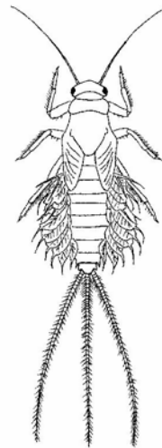
Figure 4.49: Leptophlebia sp. (Leptophlebiidae) larva, Dorsal View.
