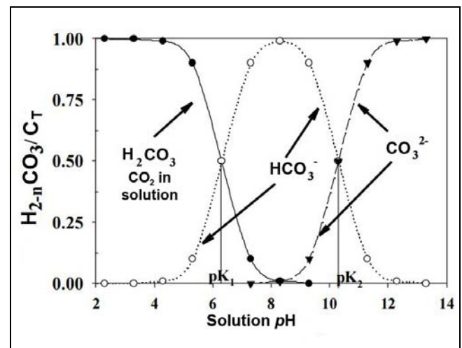
Figure 68. Distribution of carbonate species as a fraction of total dissolved carbonate in relation to solution pH. Note that H 2 CO 3 represents CO 2 dissolved in water; HCO 3 - is bicarbonate, and CO 3 2- is carbonate. Modified from Soil Chemistry 5-1 < http://lawr.ucdavis.edu/classes/ssc102/Section5.pdf >.
